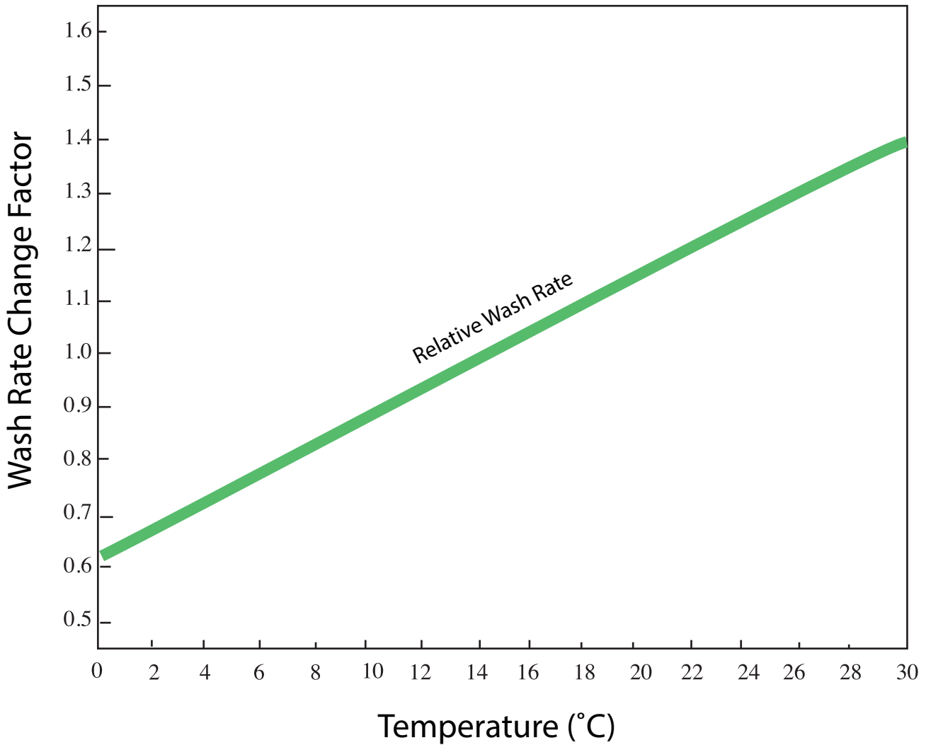
Effect of water temperature on the backwash rate for the fluidisation of a filter bed
